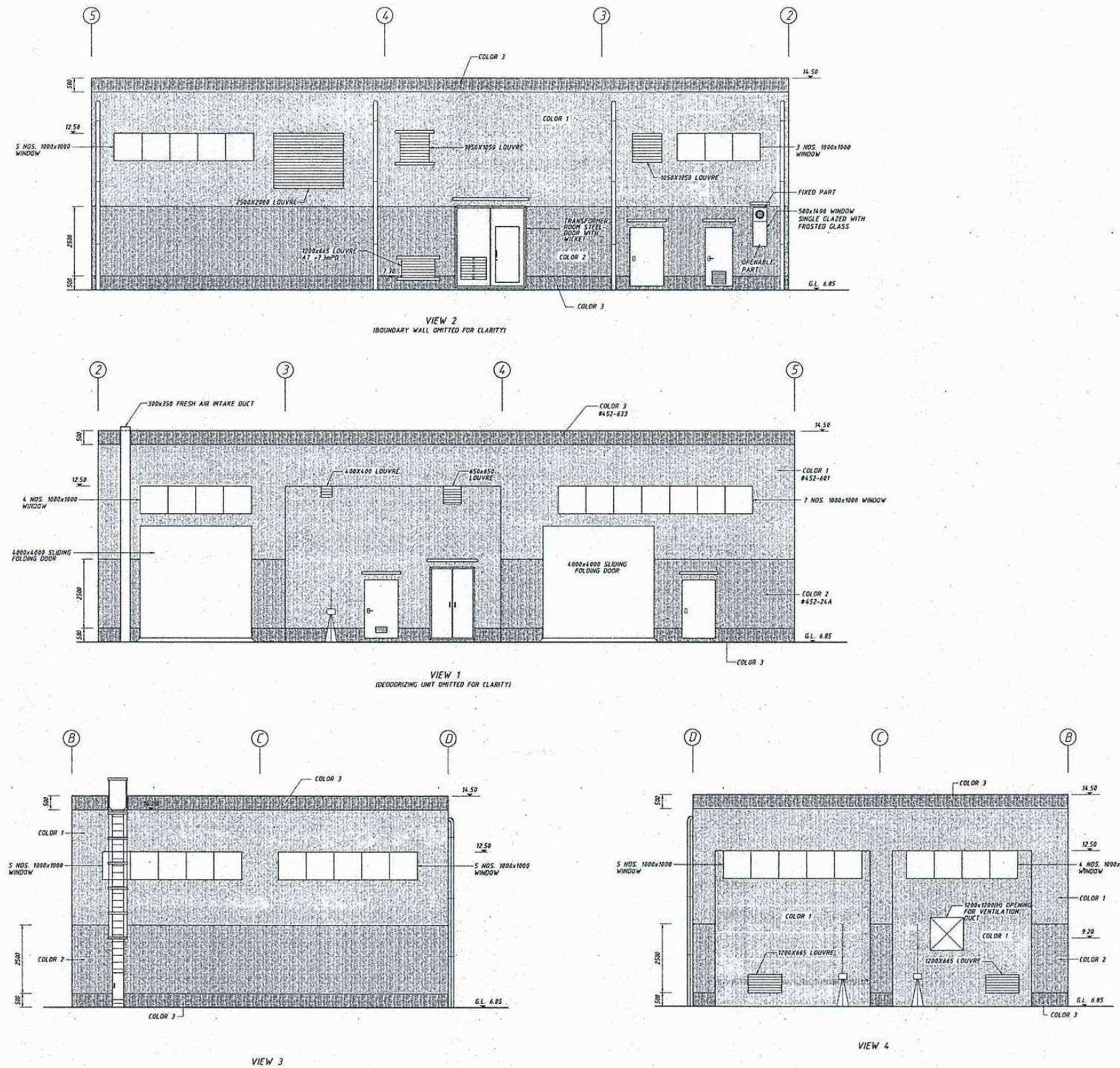
Figure 7: Sewage Pumping Station and Equalization Tanks - Architectural Elevations
